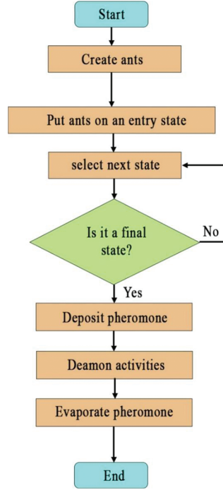
Figure 5: ACO flowchart [67]
