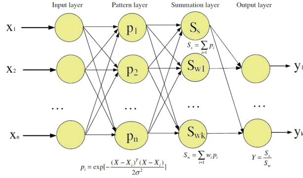
Figure 3: GRNN structure [45]
