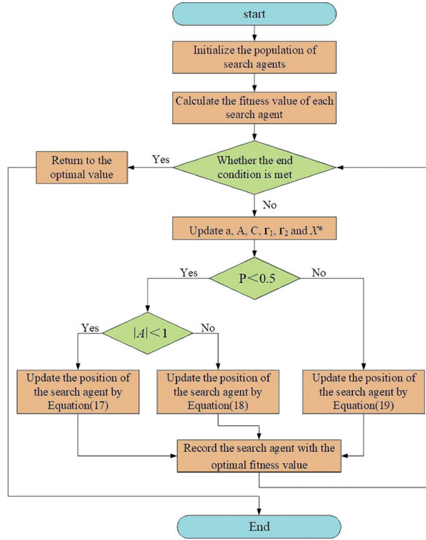
Figure 7: WOA flowchart [83]
