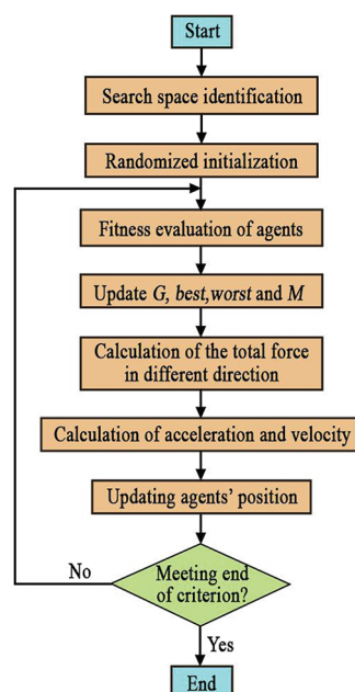
Figure 4: GSA flowchart [61]
