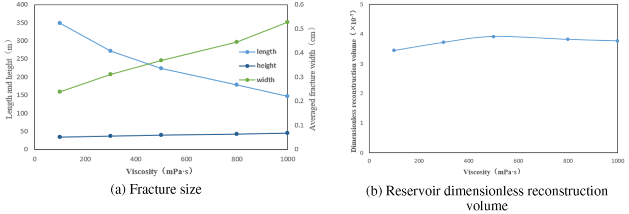
Figure 7: Fracture size and dimensionless reconstruction volume curves under different fracturing fluid viscosity
