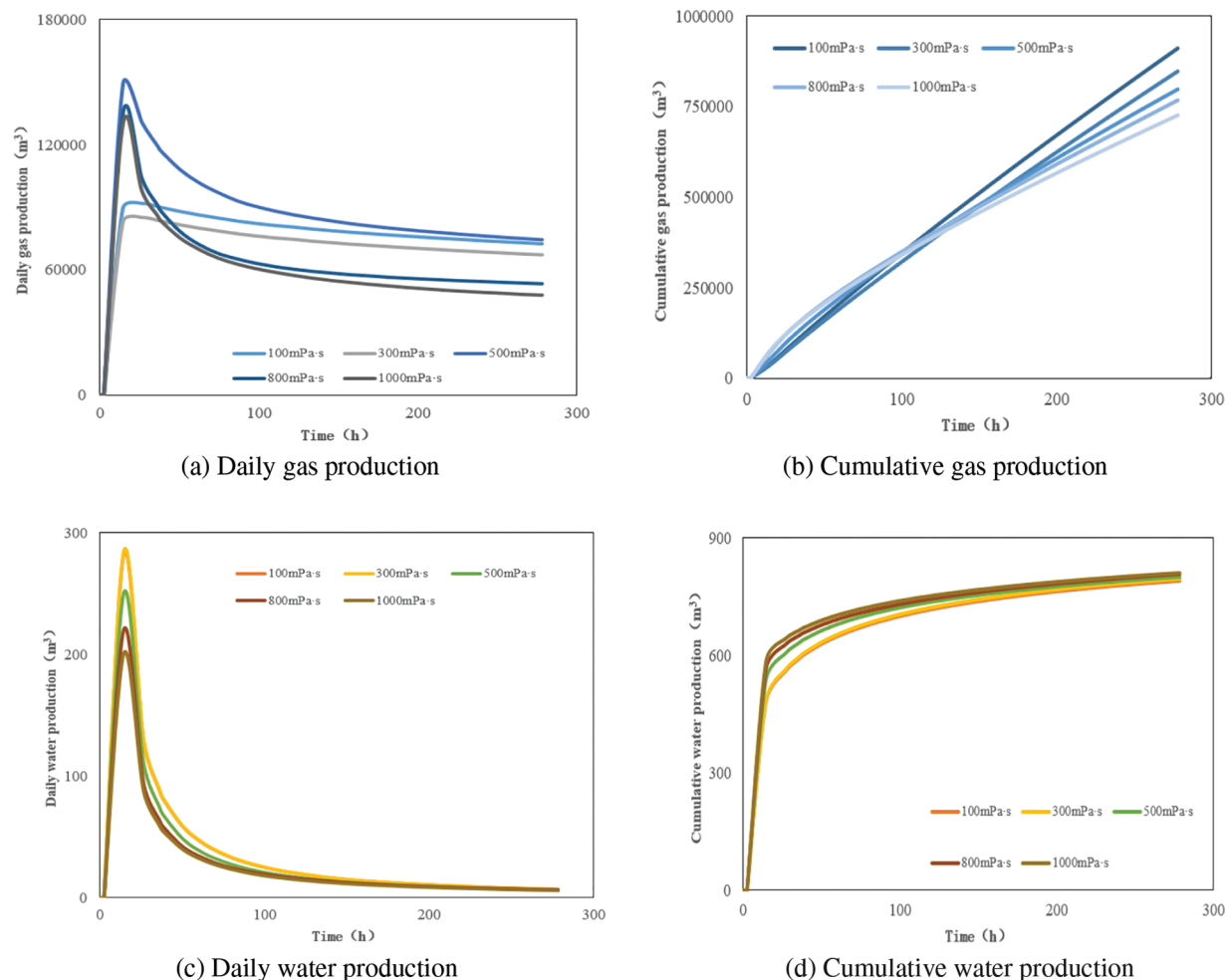
Figure 12: Gas-water production dynamics under different fracturing fluid viscosity conditions
