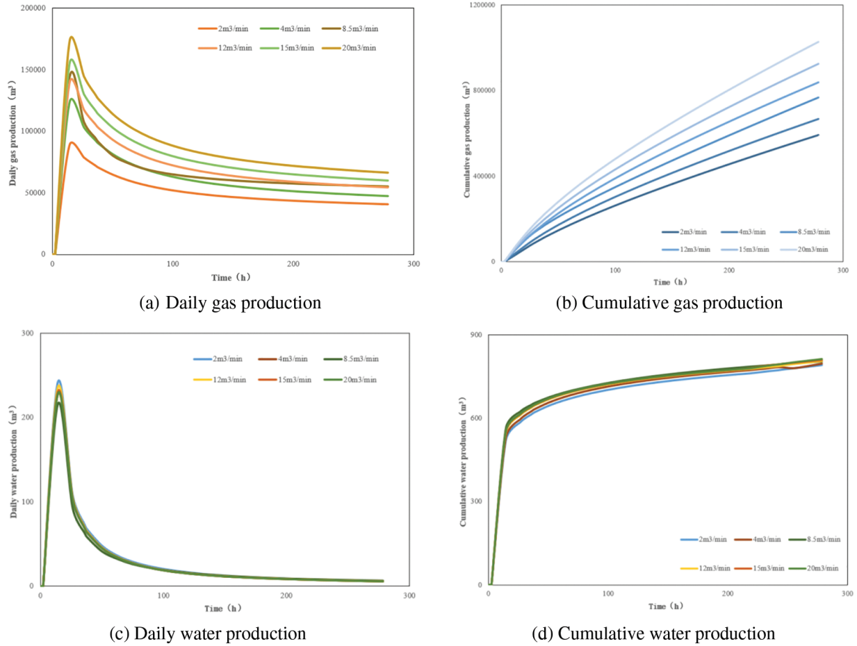
Figure 11: Gas and water production dynamics under different fracturing construction displacement conditions
