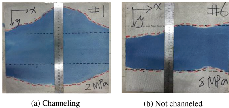
Figure 2: Fracture vertical expansion under different conditions
